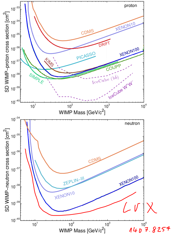
Figure 3. Results on spin-dependent WIMP-nucleon scattering cross sections, presented assuming that WIMPs would couple only to proton- or to neutron-spins. (Top) The proton-only case is dominated by results from experiments which employ a target containing ^{19}\text{F} (COUPP [48], SIMPLE [49], PICASSO [50]). The new results from the directional DRIFT detector [52] and from indirect WIMP searches by IceCube [53] are also shown. (Bottom) The best limit on neutron-only couplings is from XENON100 [54] using ^{129}\text{Xe} and ^{131}\text{Xe} as target nuclei. Figures adapted from [54], see more references there.
