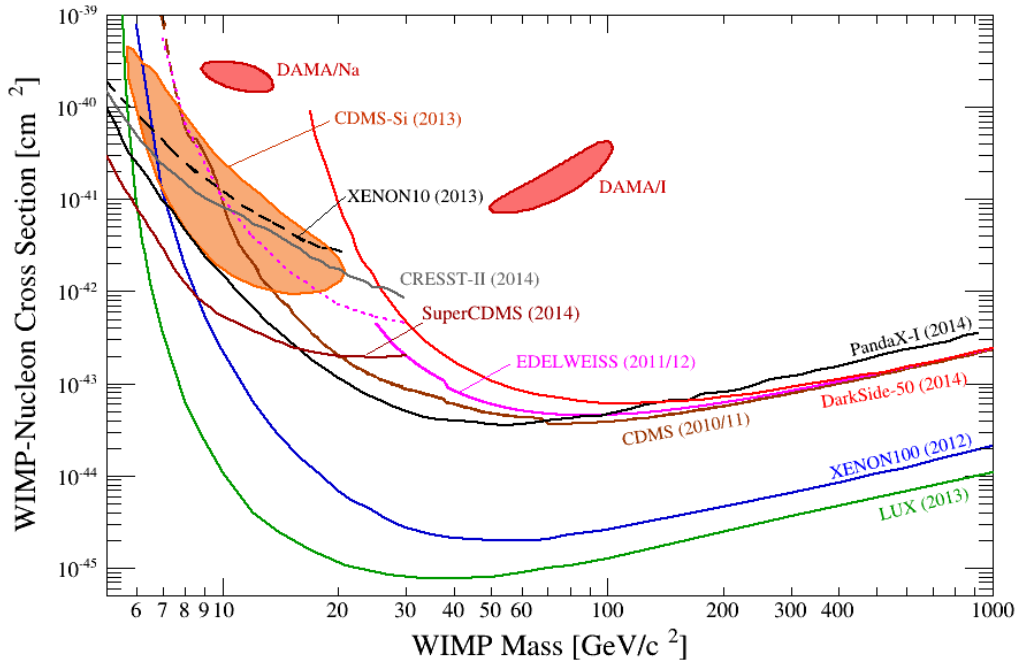
Figure 1. Results on spin-independent (scalar) WIMP-nucleon interactions as derived from direct detection experiments. The results from DAMA/LIBRA [16, 21] and CDMS-Si [19] (closed contours, see text), which could be interpreted as being induced by interactions of light-mass WIMP dark matter, are challenged by the exclusion limits (at 90% CL, lines) from many other experiments. The parameter space is currently dominated by the dual-phase liquid xenon time projection chambers (TPCs) XENON100 [11] and LUX [12]. Some results discussed in the text are not plotted to increase the readability of the plot.
